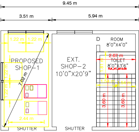
GROUND FLOOR PLAN [SOUTH FACING]
