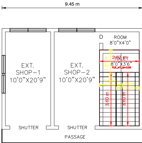
FIRST FLOOR PLAN [SOUTH FACING]
