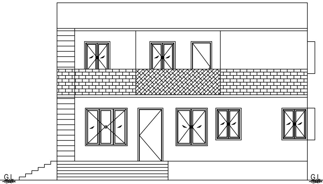
FRONT ELEVATION
