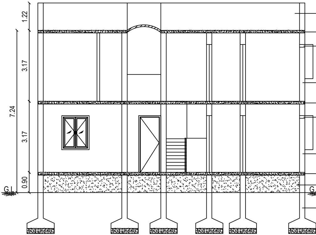
SECTION - (A-B)
