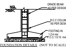
FOUNDATION DETAILS (NOT TO SCALE)
