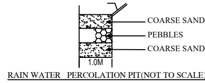
RAIN WATER PERCOLATION PIT(NOT TO SCALE)
