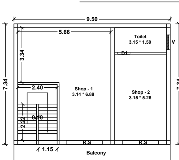
Approved & Additional Ground Floor Commercial Building
