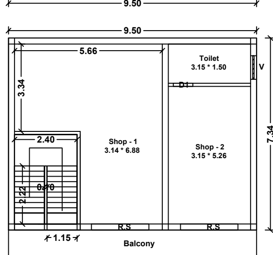
Approved & Additional First Floor Commercial Building
