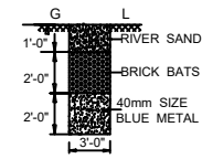
RAIN WATER PERCOLATION PIT (NTS)
