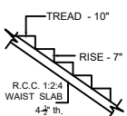
STAIRCASE DETAILS (NTS)
