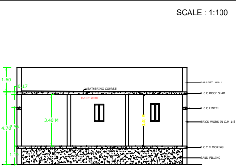
SECTION ON K-S
