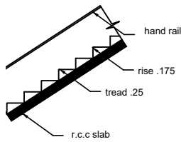
STAIR
