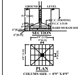
FOUNDATION DETAILS
