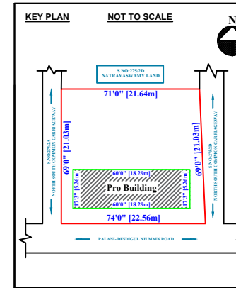
AREA DETAILS .
