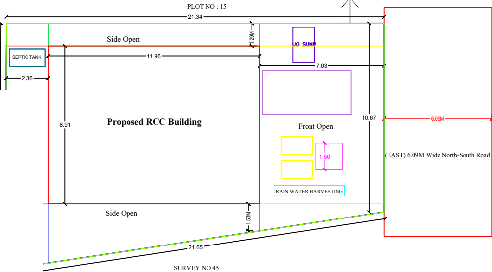
SITE PLAN
