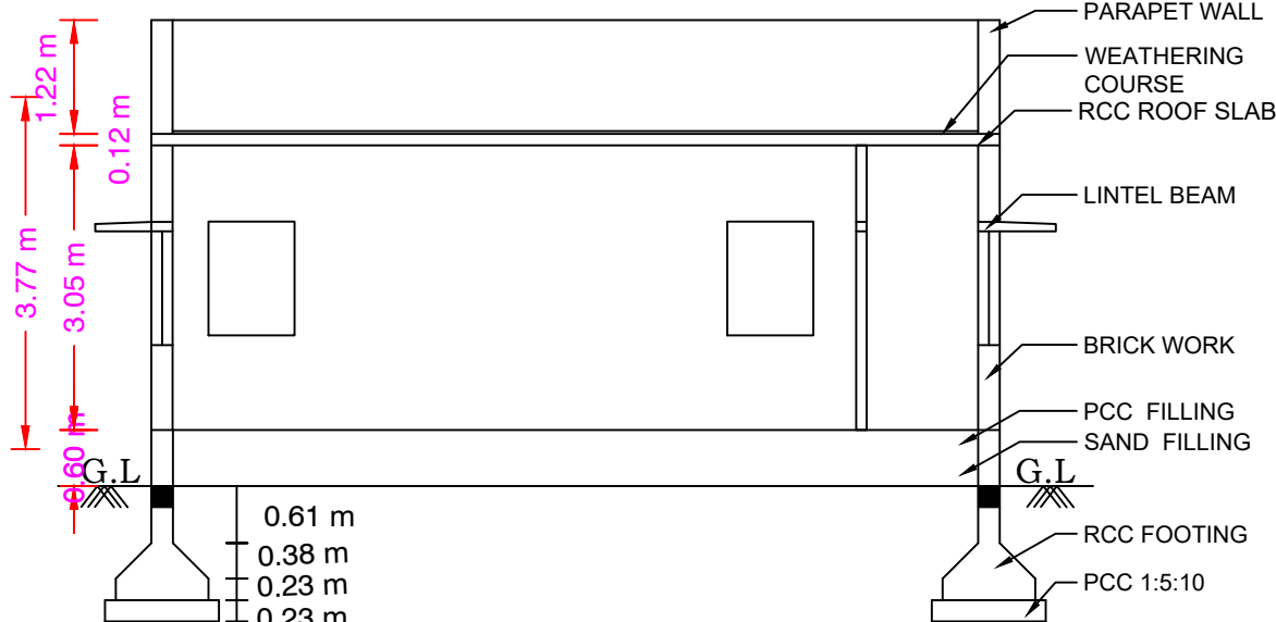
SECTION ON KA
