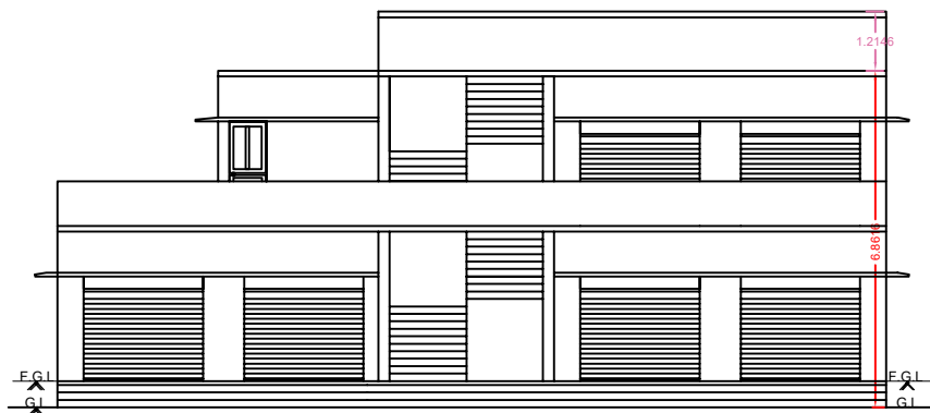
FRONT ELEVATION
