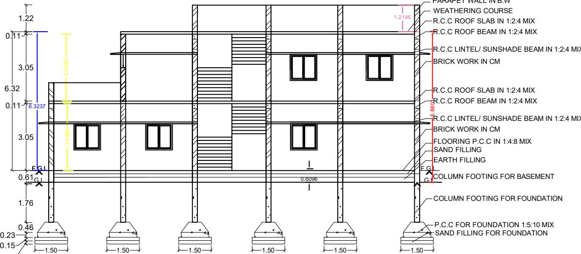
SECTION ON-AA
