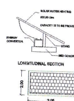
SOLAR SYSTEM
