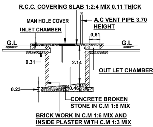
. SECTION ON SEPTIC TANK .
