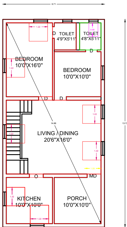
GROUND FLOOR PLAN [EAST FACING]
