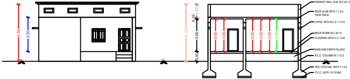
ELEVATION (FACING EAST)
