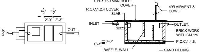
SEPTIC TANK DETAIL
