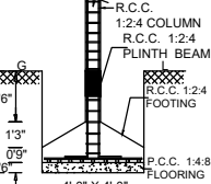
FOUNDATION DETAIL
