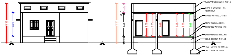
ELEVATION (FACING NORTH )
