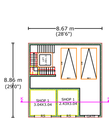
PROPOSED GROUND FLOOR PLAN COMMERCIAL BUILDING
