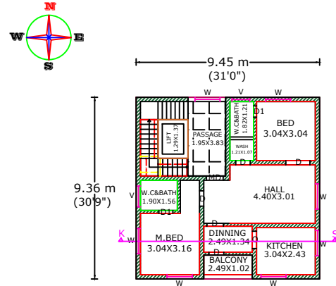
PROPOSED FIRST FLOOR PLAN RESIDENTIAL BUILDING
