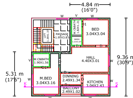
PROPOSED SECOND FLOOR PLAN RESIDENTIAL BUILDING
