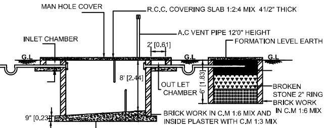
SECTION OF SEPTIC TANK AND DISPERSION TRENCH
