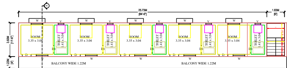
PRO-FIRST FLOOR PLAN
