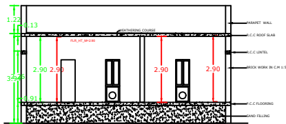
SECTION ON K-S
