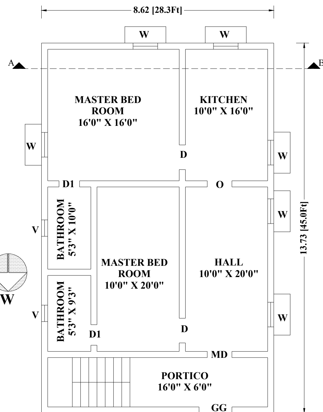
GROUND FLOOR
