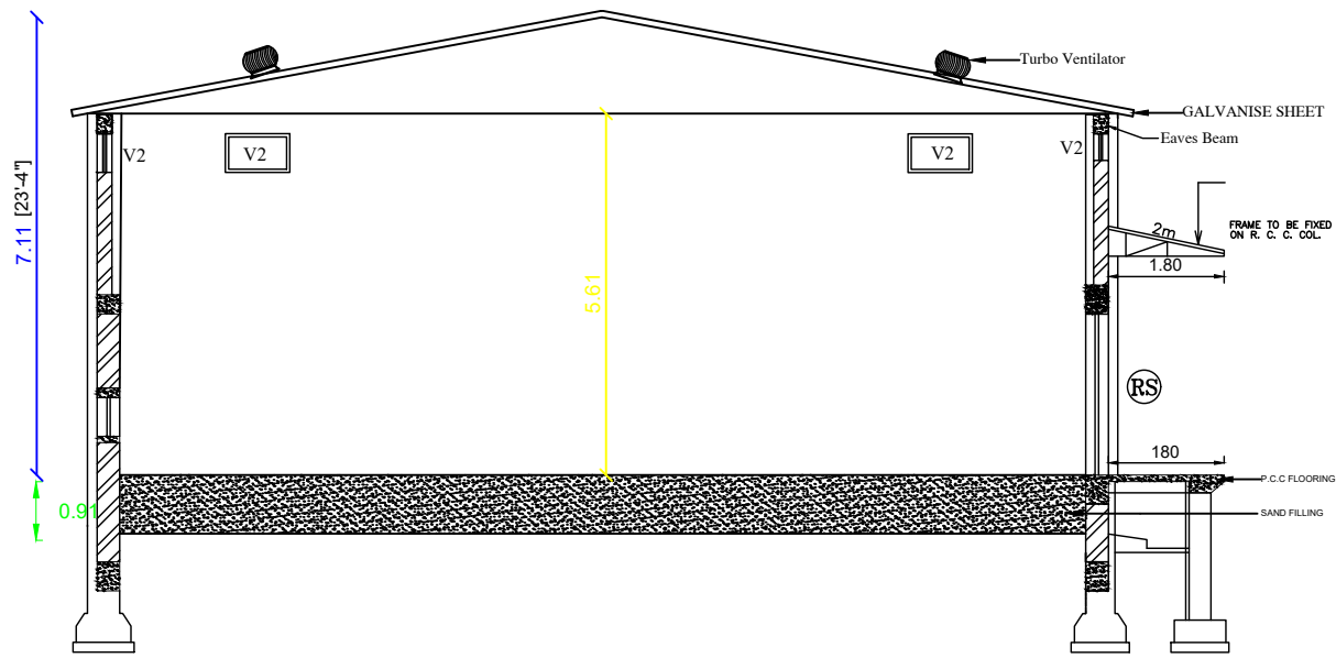
SECTION
