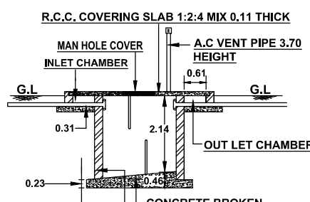
. SECTION ON SEPTIC TANK .
