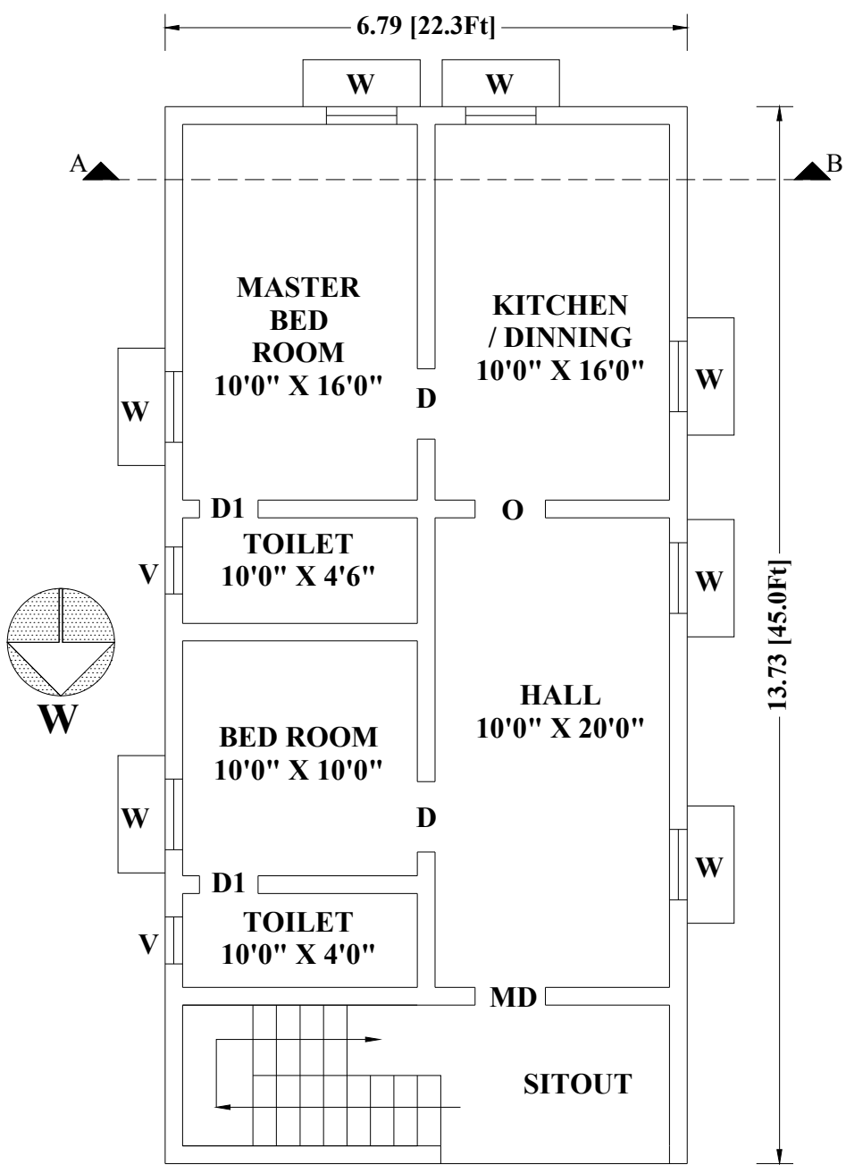
GROUND FLOOR
