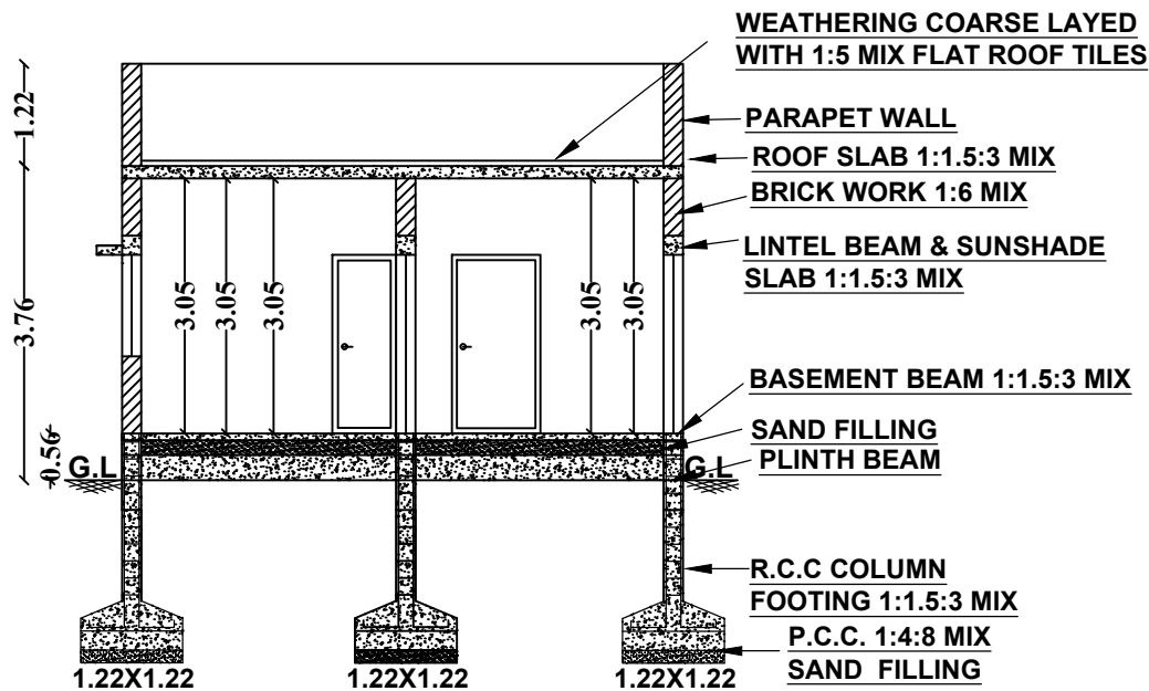
.SECTION "AB".
