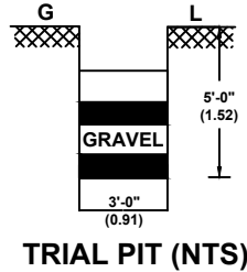
TRIAL PIT (NTS)
