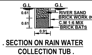
. SECTION ON RAIN WATER COLLECTION TUB .
