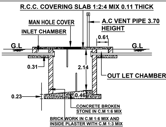
.SECTION ON SEPTIC TANK .
