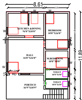
GROUND FLOOR PLAN FACING NORTH
