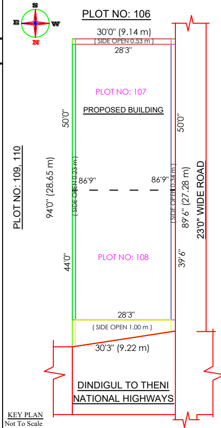
AREA DETAILS
