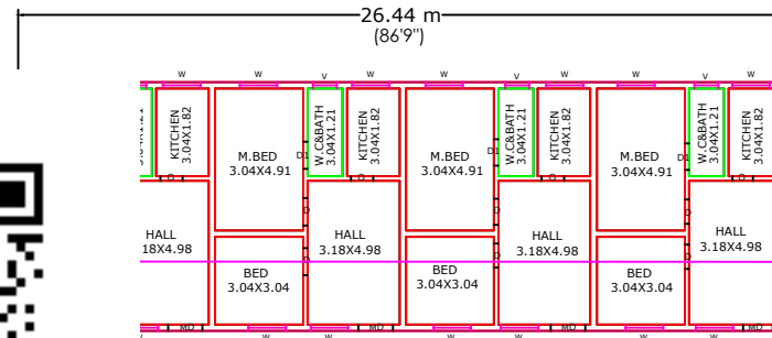
EXISTING GROUND FLOOR PLAN
