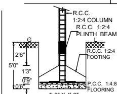
FOUNDATION DETAIL
