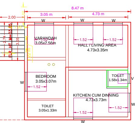
FIRST FLOOR PLAN (RESIDENTIAL)
