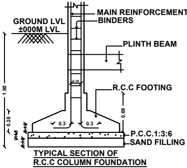
TYPICAL SECTION OF R.C.C COLUMN FOUNDATION
