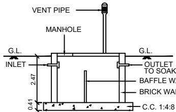
SECTION OF SEPT. TANK
