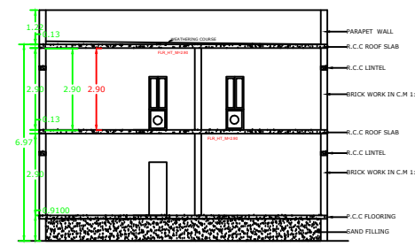
SECTION ON K-K
