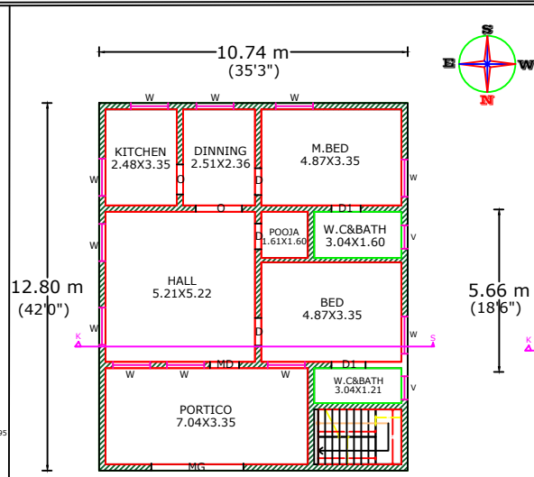
EXISTING GROUND FLOOR PLAN Already Approved
