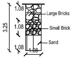
SECTION OF RAIN WATER
