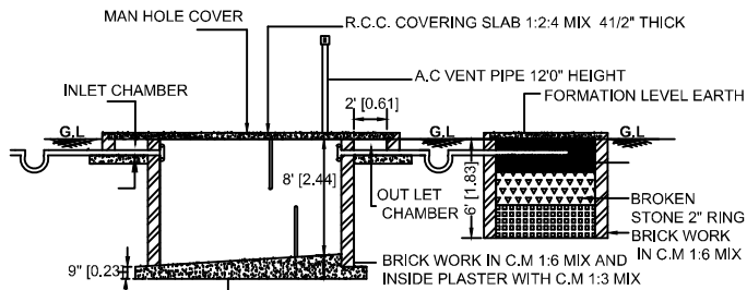
SECTION OF SEPTIC TANK AND DISPERSION TRENCH
