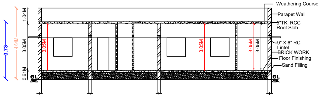
SECTION ON "BC"
