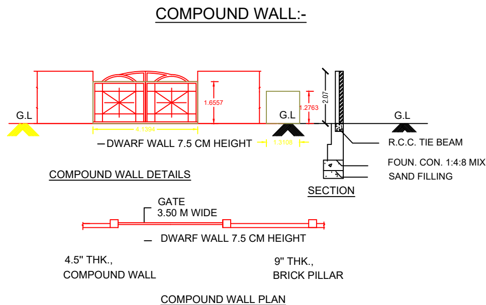
COMPOUND WALL PLAN
