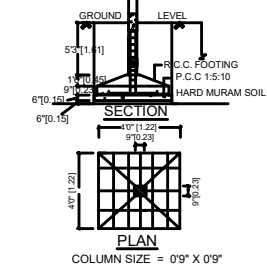
FOUNDATION DETAILS
