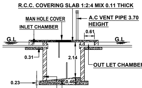
RAIN WATER HARVESTING DETAIL (NOT TO SCALE)
