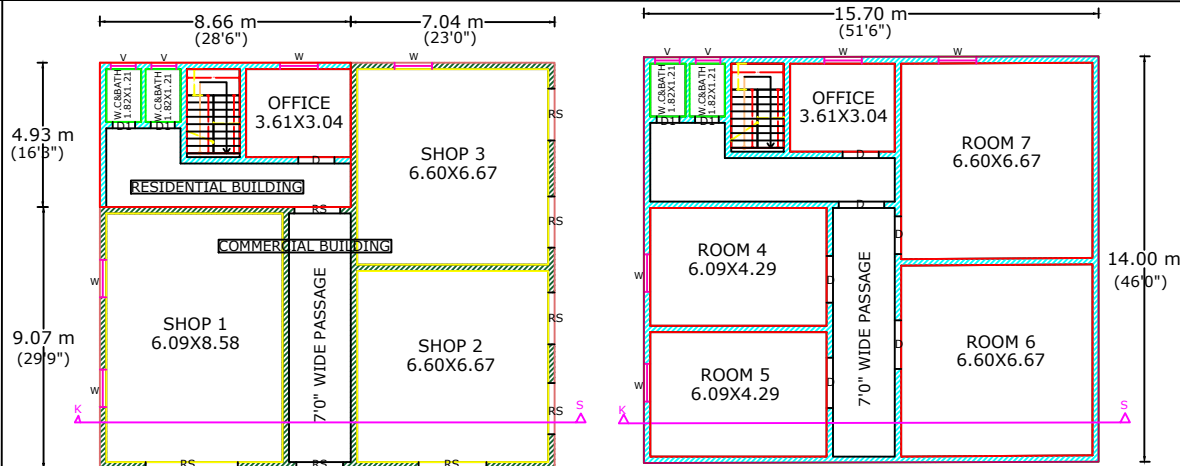
PROPOSED GROUND FLOOR PLAN COMMERCIAL BUILDING PROPOSED GROUND FLOOR PLAN RESIDENTIAL BUILDING
