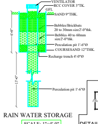
RAIN WATER STORAGE SCALE: 1"=4'-0"
