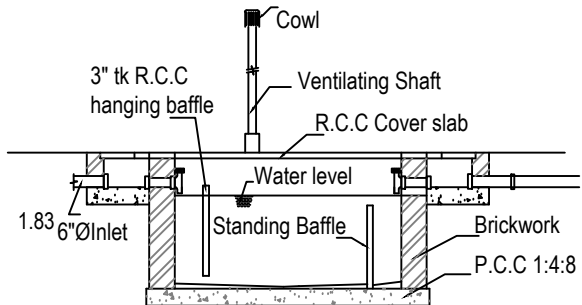
SECTION DETAILS OF SEPTIC TANK
