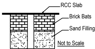
SECTIONAL ELEVATIONAL FOR RAIN WATER RECHARGEABLE TANK
