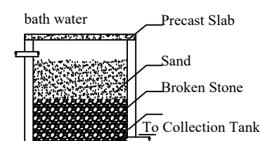
Section of Filter Unit
