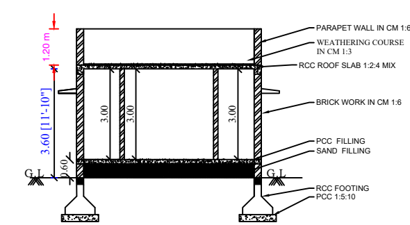
SECTION - "SR"
