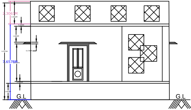
FRONT ELEVATION
