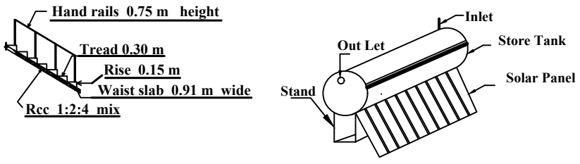
Staircase Details
