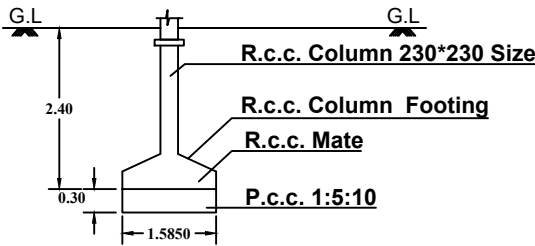
Foundation Details
