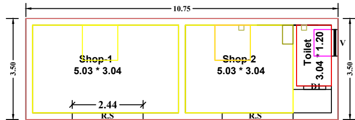
ADDITIONAL GROUND FLOOR - SHOP BUILDING
