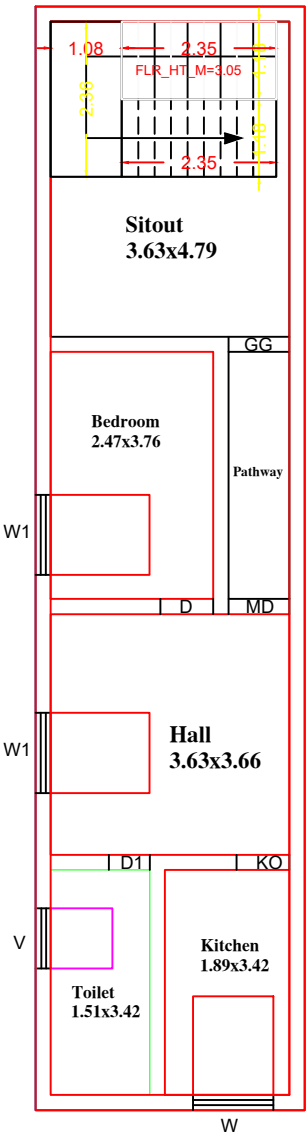
SECOND FLOOR
