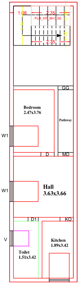
FIRST FLOOR
