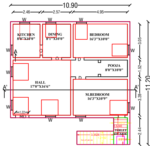
GROUND FLOOR PLAN FACING NORTH
