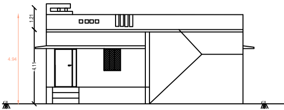
ELEVATION FACING NORTH
