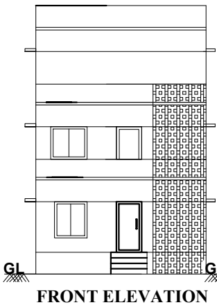
FRONT ELEVATION
