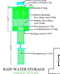
RAIN WATER STORAGE
