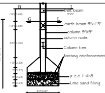
FOUNDATION DETAILS
