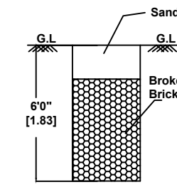
RAIN WATER HARVESTING RECHARGE PIT DETAILS (NOT TO SCALE)
