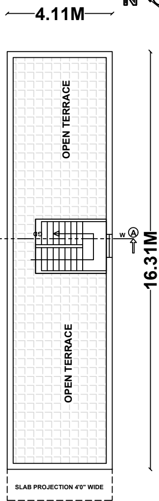
TERRACE FLOOR PLAN
