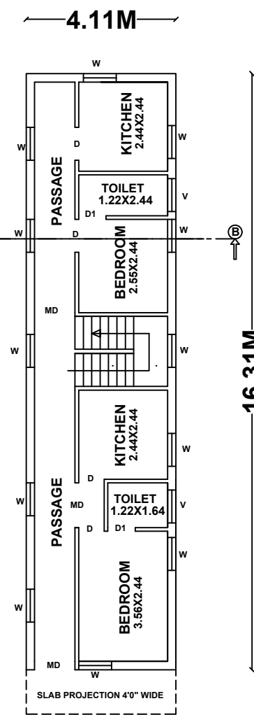
PRO.SECOND FLOOR PLAN
