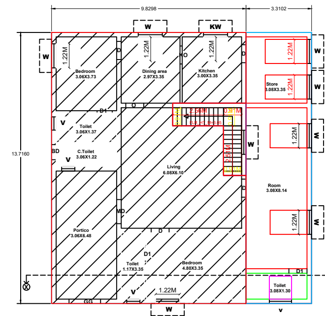
EXISTING AND ADDITIONAL PROPOSED GROUND FLOOR PLAN
