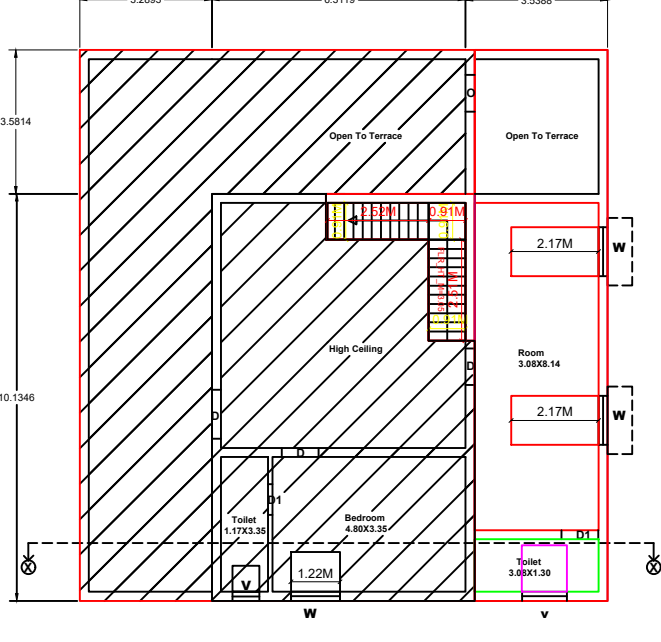
EXISTING AND ADDITIONAL PROPOSED FIRST FLOOR PLAN
