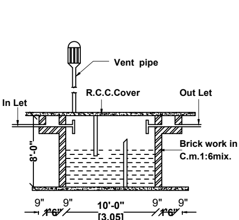
SEPTIC TANK DETAILS (NOT TO SCALE)
