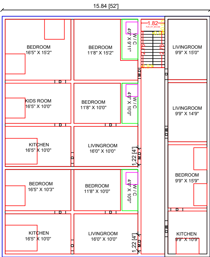
PROPOSED SECOND FLOOR
