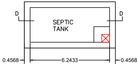
PLAN OF SEPTIC TANK SCALE 1"=2'0"
