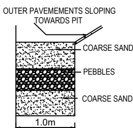
RAIN WATER PERCOLATION BED
