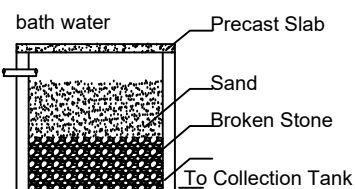
Section of Filter Unit
