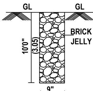
PERCOLATION PIT
