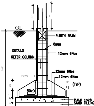
FOUNDATION DETAILS
